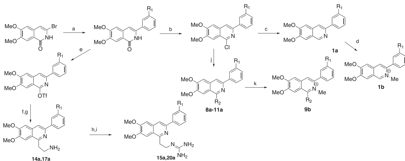
Scheme 1. Synthesis of 3-phenylisoquinolines from 6,7-dimethoxy-3-bromoquinolin-1-one. Reagents and conditions: (a) R 1 -C 6 H 4 (OH) 2 , Pd(OAc) 2 , XPhos, K 2 CO 3 , ACN/H 2 O, 100 °C; (b) POCl 3 , 110 °C; (c) H 2 , Pd/C (10%), EtOH, rt; (d) MeI, sealed tube 100 °C; (e) Tf 2 O, Et 3 N, DCM, −78 °C; (f) potassium t -butyl- N -[2-(trifluoroboranyl)ethyl]carbamate, PdCl 2 (dppf), Cs 2 CO 3 , dioxane/H 2 O, 102 °C; (g) TFA, DCM, 0 °C to rt; (h) 1,3-di-Boc-2-(trifluoromethylsulfonyl) guanidine, Et 3 N, CH 2 Cl 2 , 37 °C; (i) TFA, DCM, 0 °C to rt; (j) R 2 N, t -BuXPhos precatalyst, LHMDS, rt; for 8a and 9a ; R 2 N, t -BuXPhos precatalyst, NaH/DMSO, rt for 10a ; CuCN, DMSO, 140 °C; for 11a ; (k) MeI, sealed tube 100 °C.
