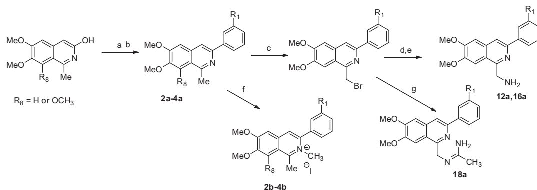
Scheme 2. Synthesis of 3-phenylisoquinolines from 6,7-dimethoxy-3-hydroxy-1-methylisoquinoline. Reagents and conditions: (a) \text{TiF}_2 , \text{Et}_3\text{N} , DCM, -78^\circ\text{C} ; (b) \text{R}_1\text{-C}_6\text{H}_4\text{B}(\text{OH})_2 , \text{Pd}(\text{OAc})_2 , XPhos, \text{K}_2\text{CO}_3 , dioxane/ \text{H}_2\text{O} , 102^\circ\text{C} ; (c) NBS, AIBN, \text{CCl}_4 , 85^\circ\text{C} ; (d) \text{NaN}_3 , DMF, rt; (e) \text{PPh}_3 polymer bound, THF/ \text{H}_2\text{O} , 0^\circ\text{C} to rt; (f) MeI, sealed tube 100^\circ\text{C} ; (g) acetamidinium HCl, \text{K}_2\text{CO}_3 , DMF, rt.
